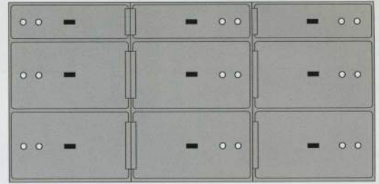
SD or SS 9 (Wt. 149 lbs.) 3 openings ea. 3" x 10" and 6 openings ea. 6" x 10"
