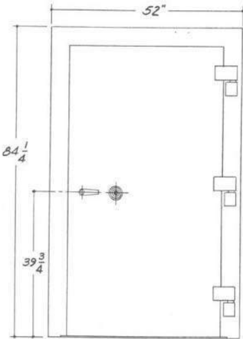
CLASS 5 VAULT DOOR
