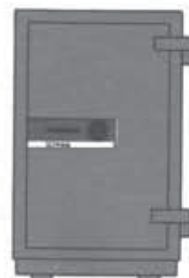
Model 1830-AN Inside 18W x 30H x 18D Overall 30 1/2W x 44 1/2H x 31 1/2D Cu. In. Capacity 10,198
